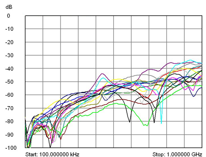
40-747-511/521 (50 Ω) Typical Isolation plots for each input channel.
