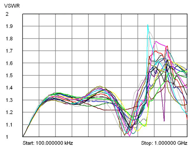
40-747-751 (75 \Omega ) Typical VSWR plots for each channel.
