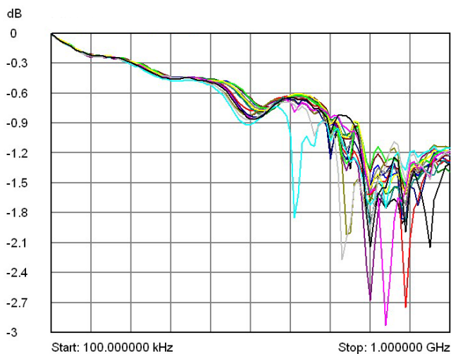
40-747-751 (75 \Omega ) Typical insertion loss plots for each channel.
