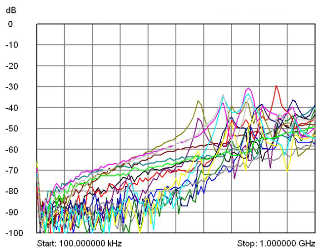
40-747-751 (75 \Omega ) Typical crosstalk between neighboring multiplexer channels.
