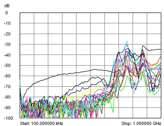
40-747-751 (75 \Omega ) Typical Isolation plots for each input channel.
