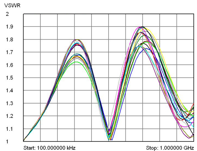
40-747-511/521 (50 Ω) Typical VSWR plots for each channel.
