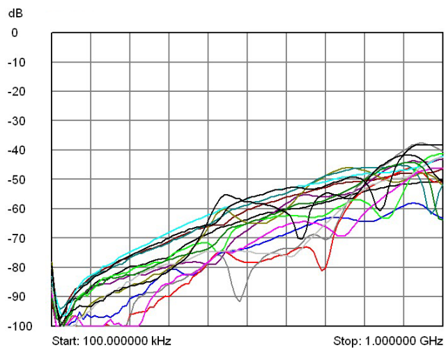
40-747-511/521 (50 Ω) Typical crosstalk between neighboring multiplexer channels.
