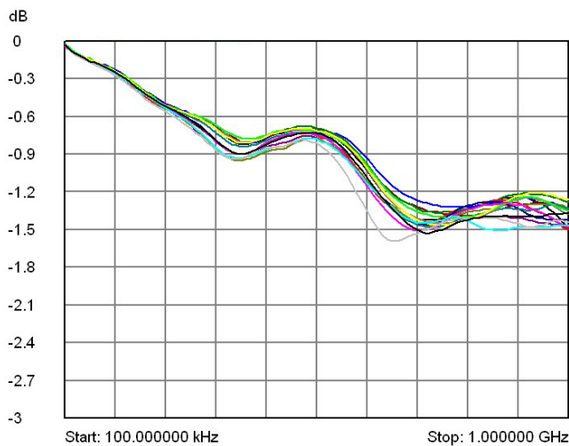
40-747-511/521 (50 Ω) Typical insertion loss plots for each channel.
