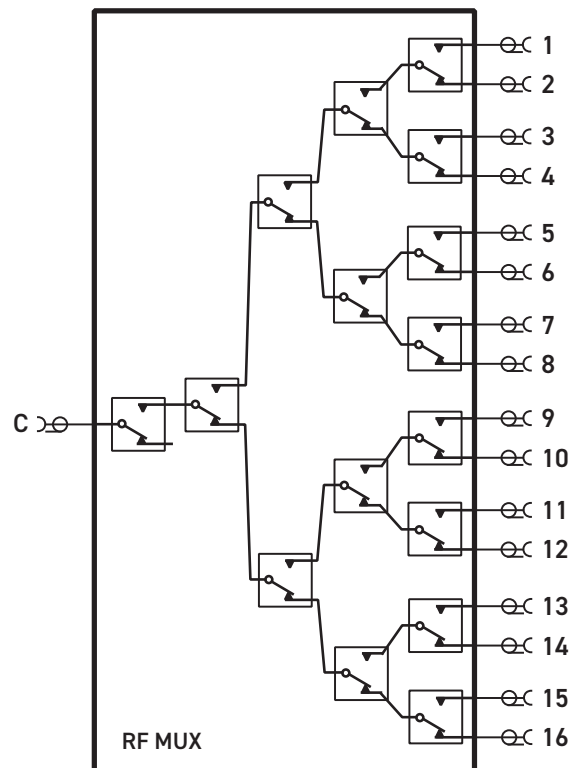
40-747 Single 16 to 1 RF MUX Switching Diagram (Default Switch Paths Shown)
